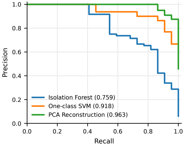
Broach dataset baseline PR curves
