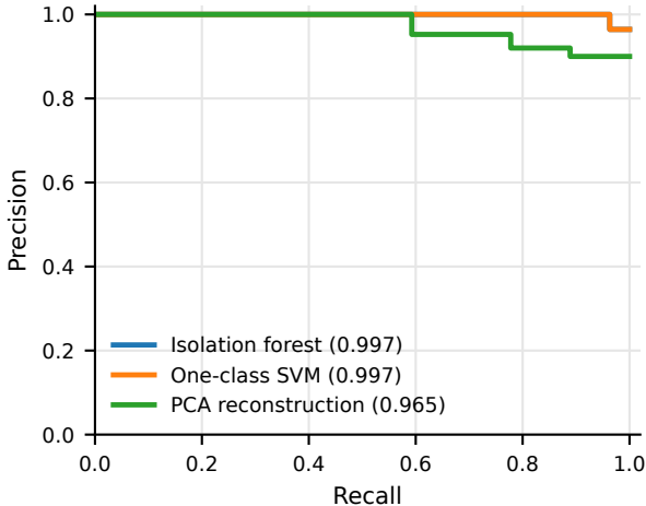
Interpolated precision-recall curves
