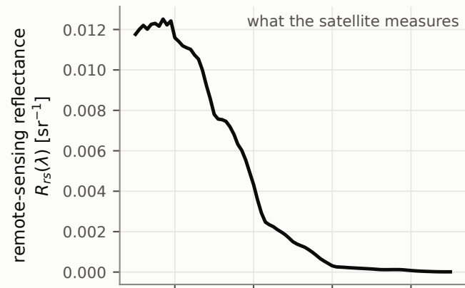
turbid water — L23 body 2949, chlorophyll 7.09 mg m -3
