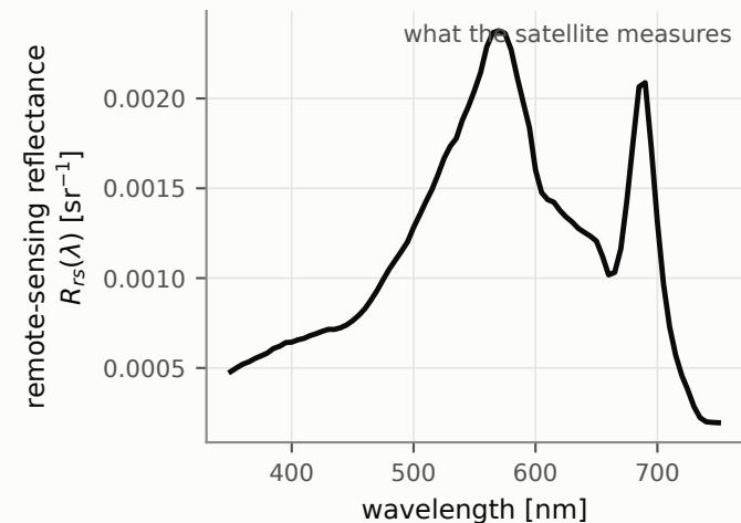
turbid water — L23 body 2949, chlorophyll 7.09 mg m -3
