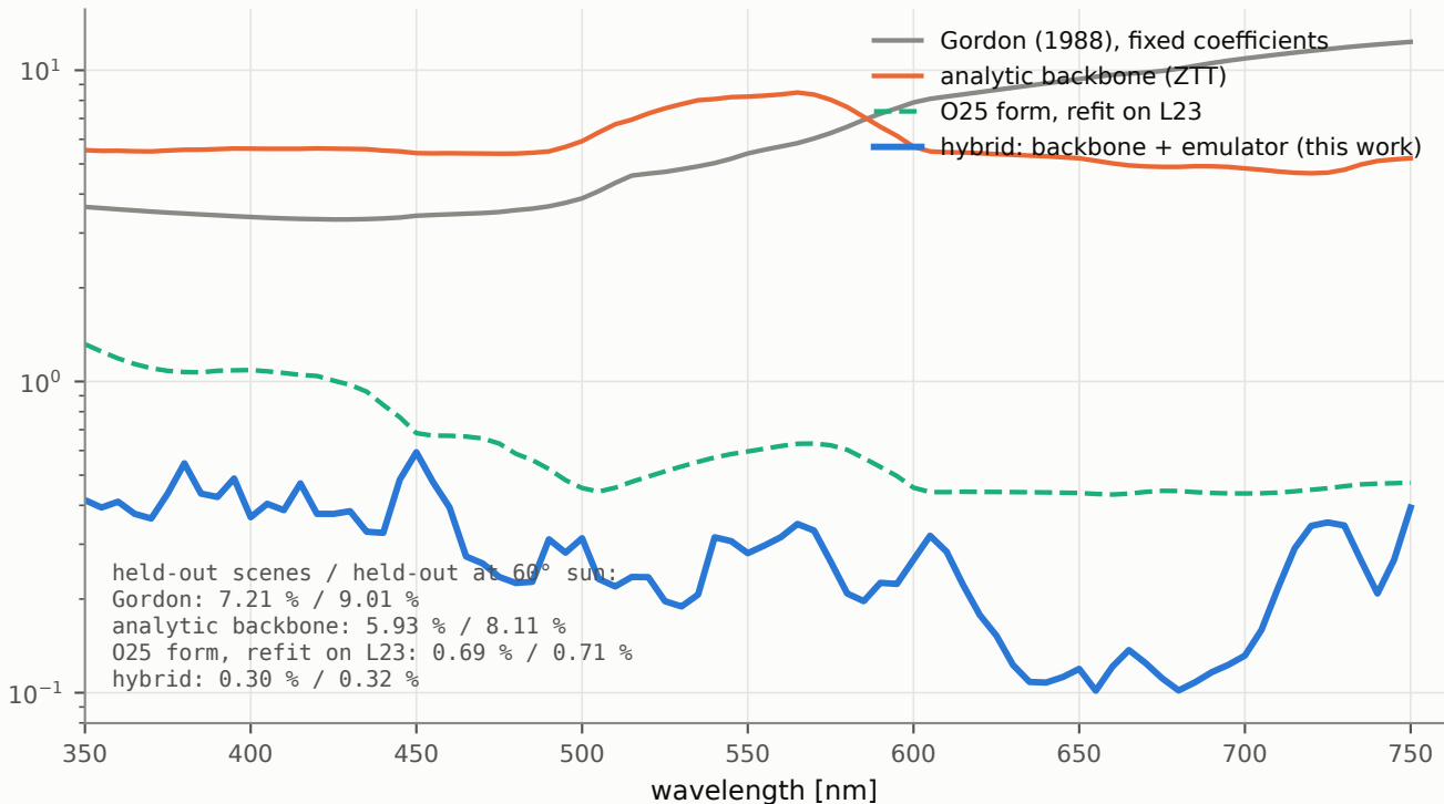
Forward model accuracy on 9,960 synthetic water bodies (train + held-out)
