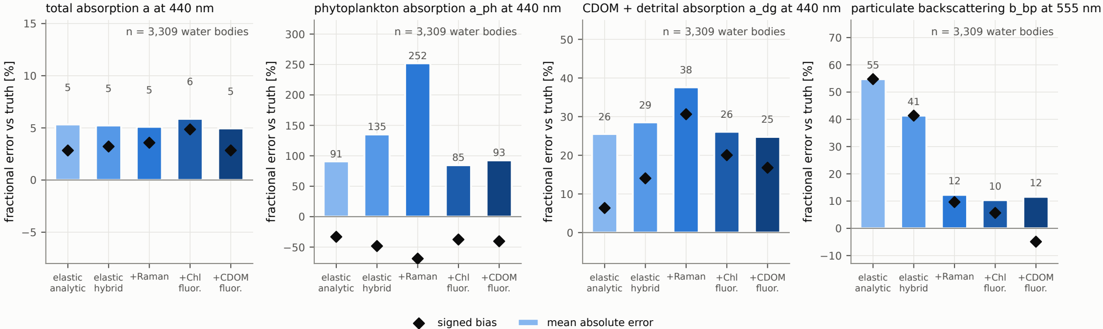
Five forward models, one parameterization, L23 synthetic truth — error moves down the ladder only where the physics was the problem
