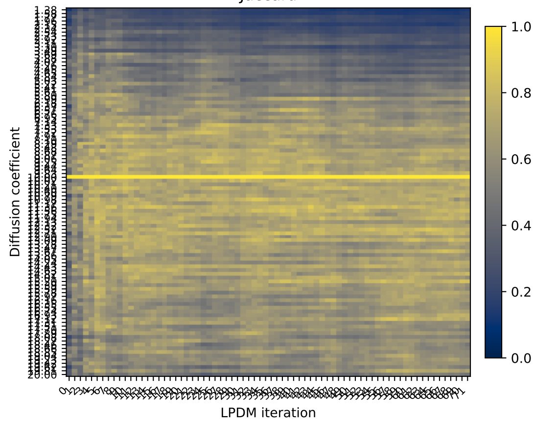
Jaccard
