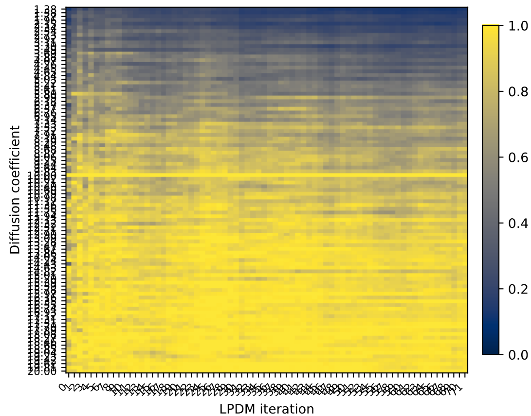
Jaccard
