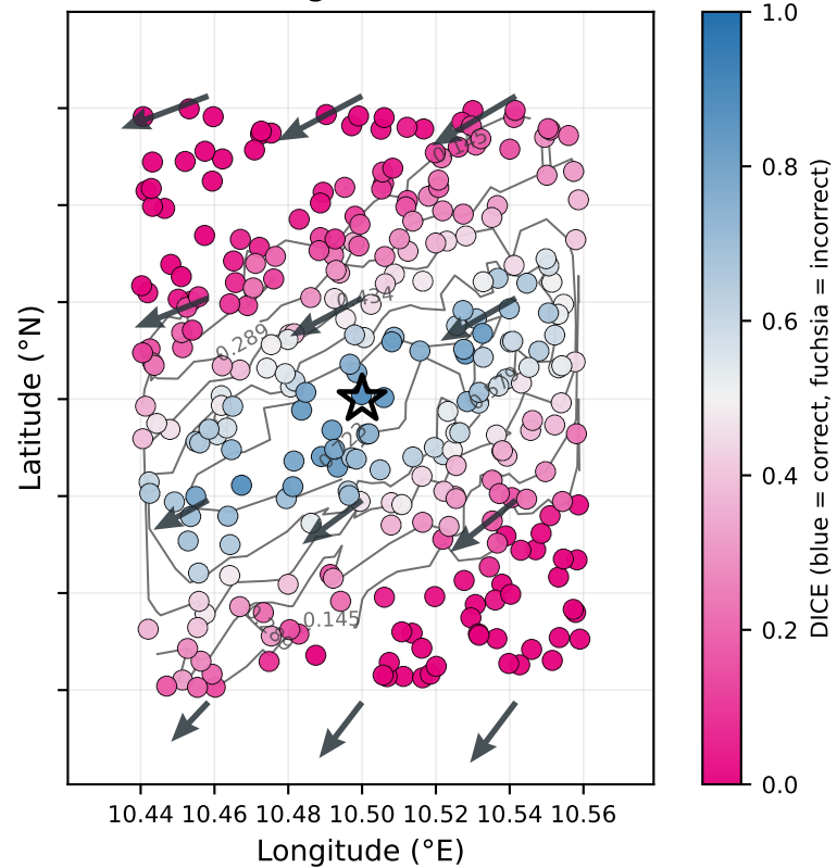
DICE (higher is better)
