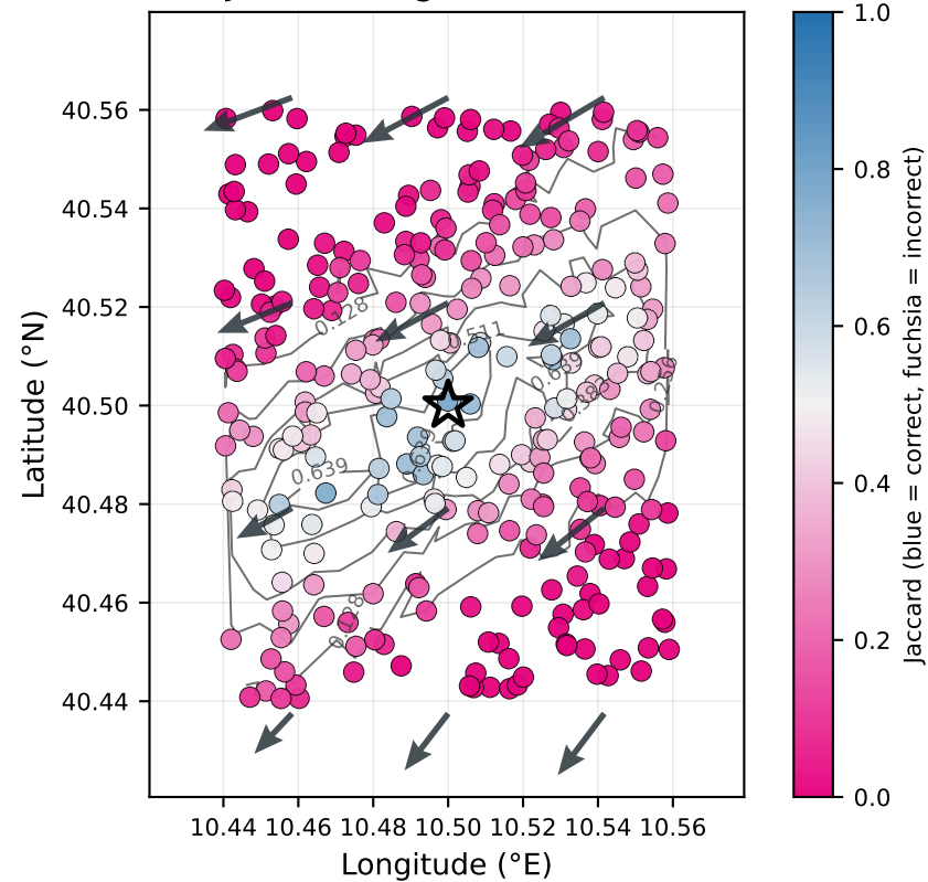
Jaccard (higher is better)
