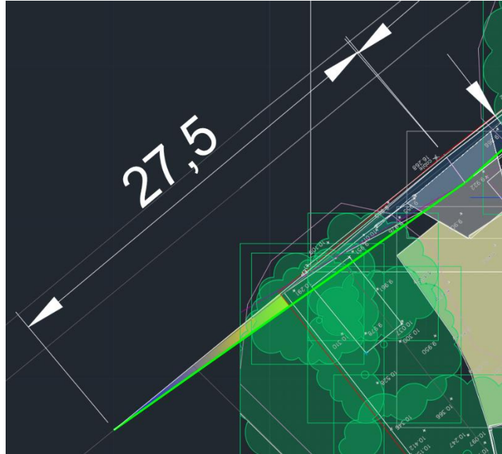
Extent of visibility splay on third party land to the west of the access
