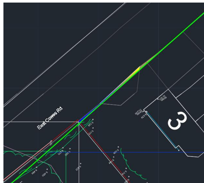
Extent of visibility splay on third party land to the east of the access
