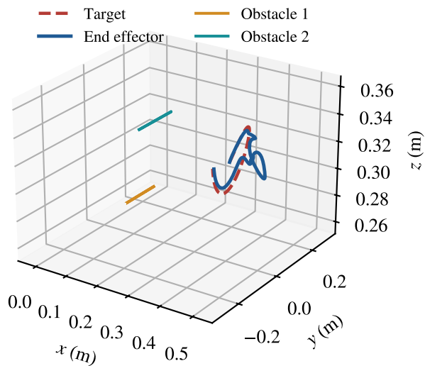
(a) Cartesian trajectories
