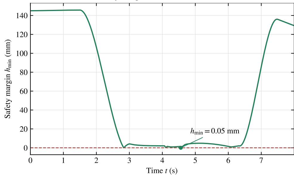
(c) Minimum CBF safety margin
