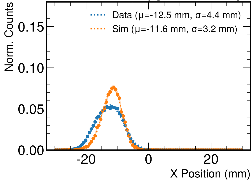
X Center of Gravity [PRELIMINARY]
