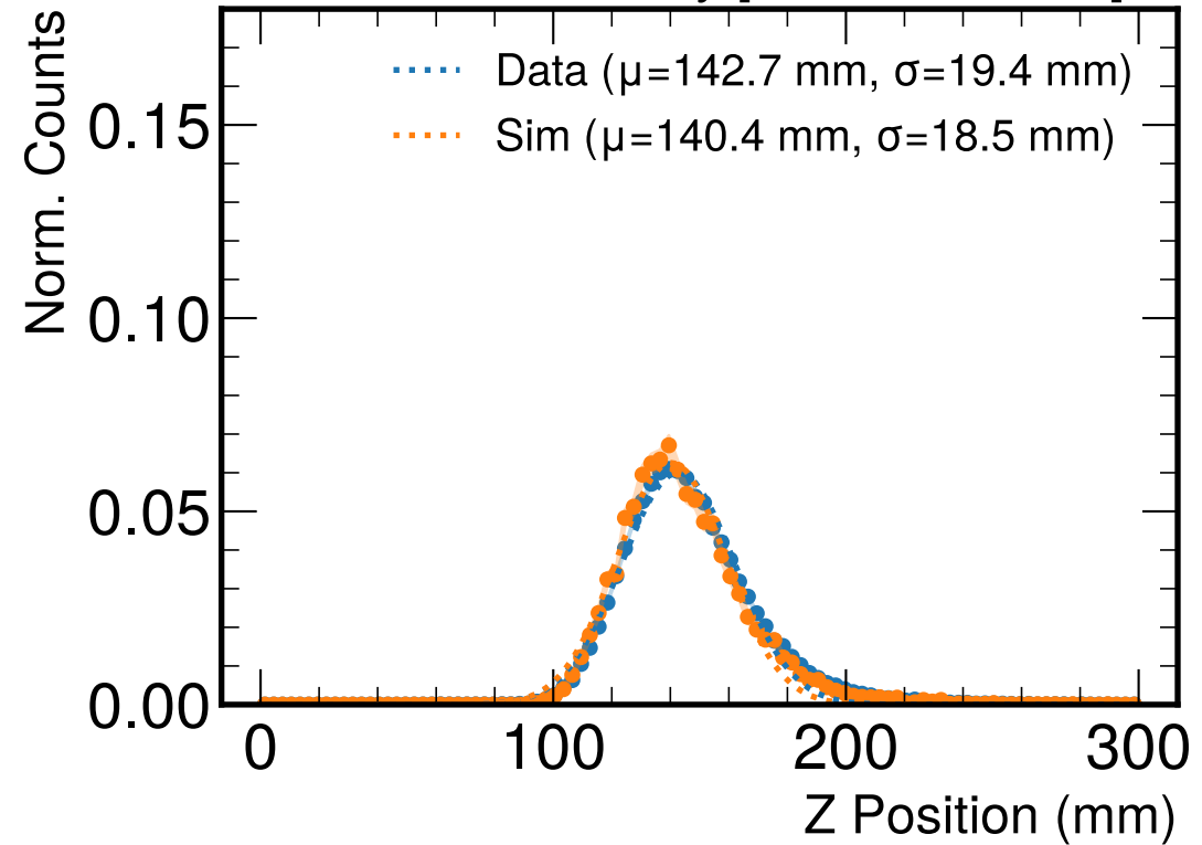
Z Center of Gravity [PRELIMINARY]
