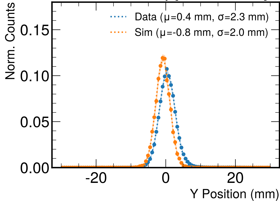
Y Center of Gravity [PRELIMINARY]
