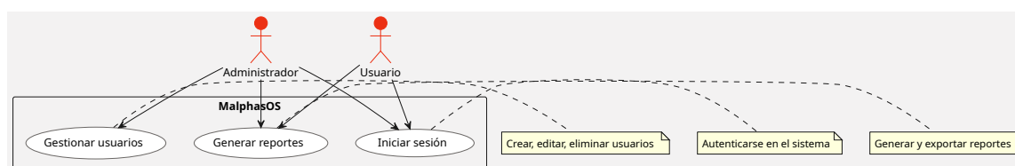
Figure 3: CU - MalphasOS General
