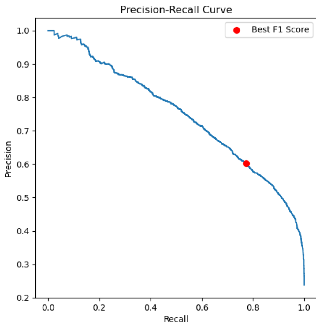
Figure 5: Precision Recall Curve
