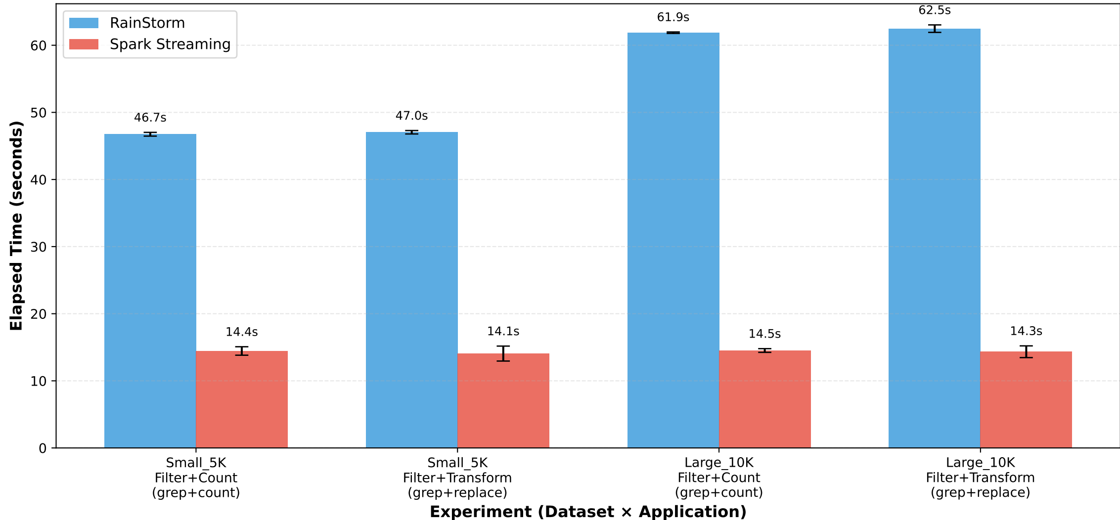
RainStorm vs Spark Streaming: Processing Time Comparison
