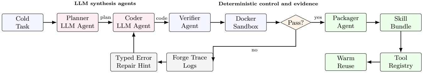
Figure 2: Internal multi-agent forge pipeline. Planner and Coder perform LLM synthesis; Verifier, Docker sandbox, Packager, and registry insertion provide deterministic control and evidence logging.
