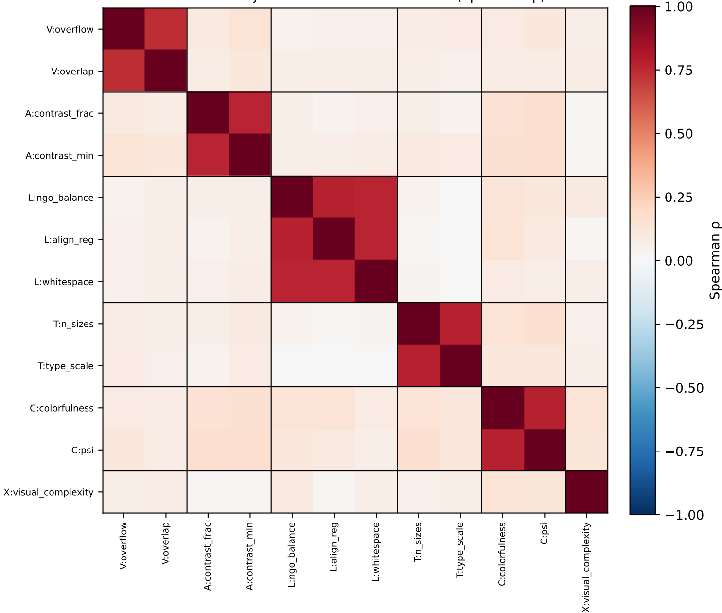
F4 · Which objective metrics are redundant? (Spearman \rho )
