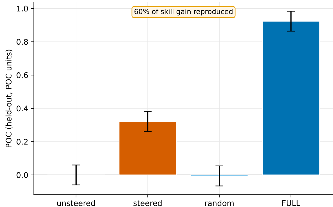
F8 · Does the direction steer with no prompt? (held-out causal test)
