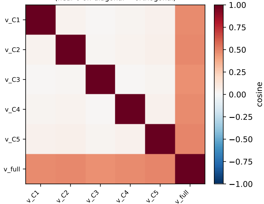
cosine among sub-directions (near-0 off-diagonal \Rightarrow orthogonal)
