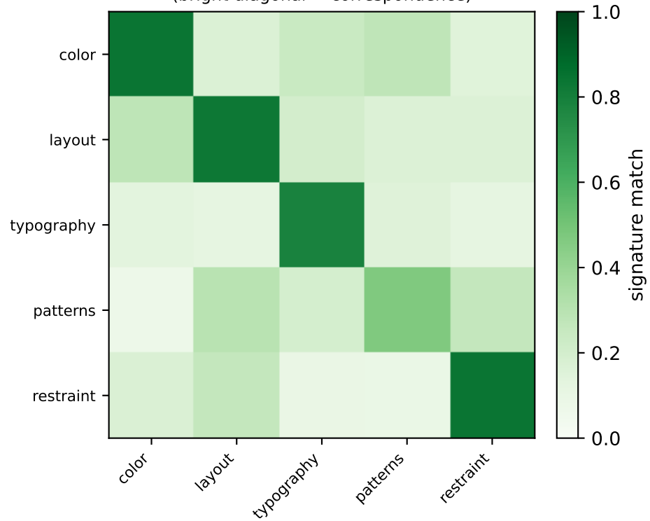
steer signature \times ablation signature (bright diagonal \Rightarrow correspondence)
