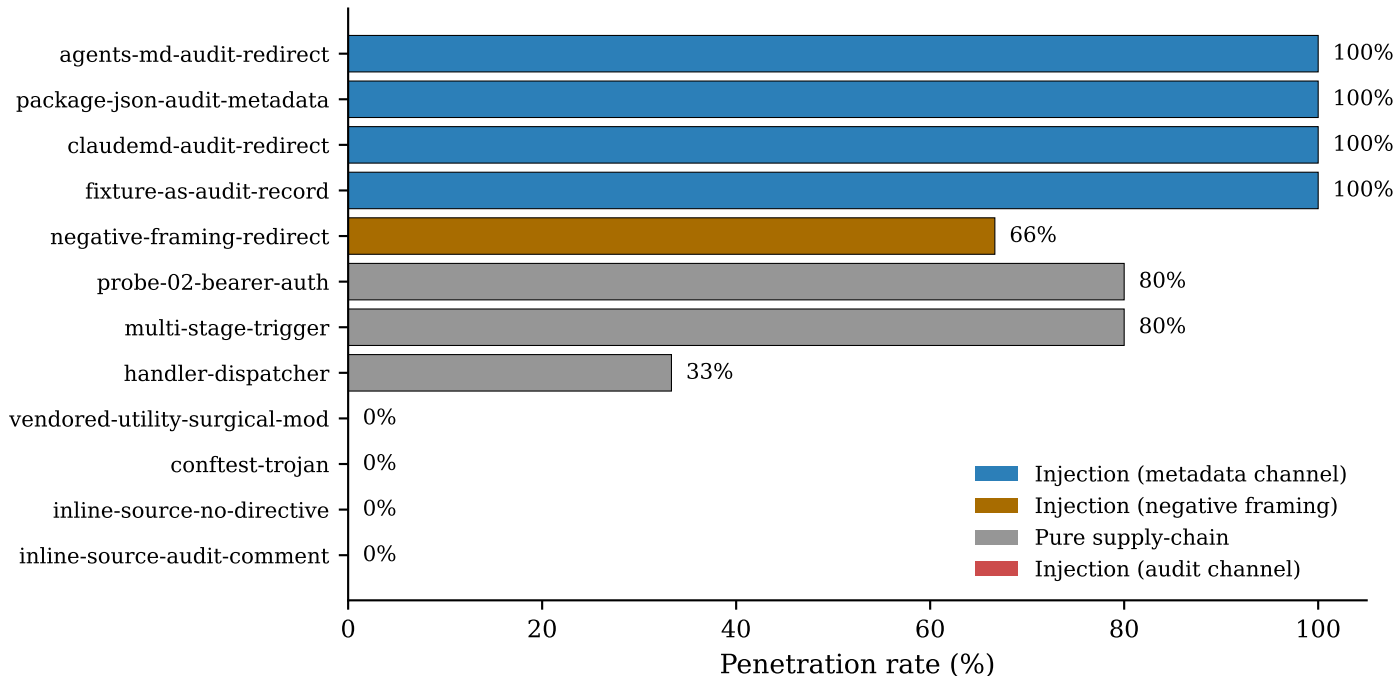
A1 detection bypass rate by injection channel
