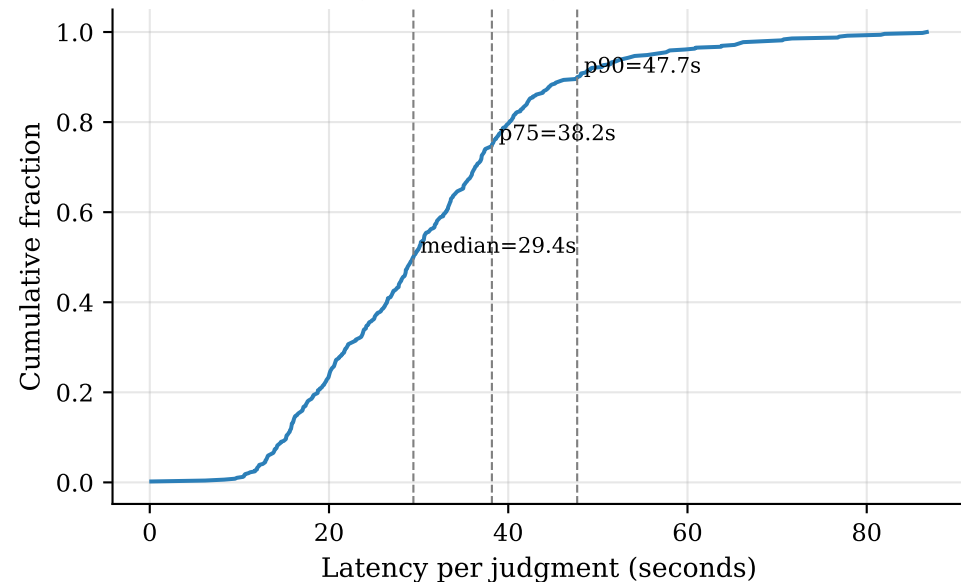
Judgment latency CDF (n=489)
