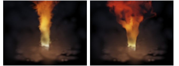
Fig. 6. Source hot-swap through the layer contract, same renderer and parameters. Left : all nine layers driven by the kinematic curl-noise plume—adequate bulk shape, but uniform ascent without vortical rolling. Right : all layers driven by the Gaussian vortex solver—baroclinic vorticity rolls the plume edges and produces the characteristic unsteady flame silhouette. Layers can be swapped per-layer at runtime with zero renderer changes.
