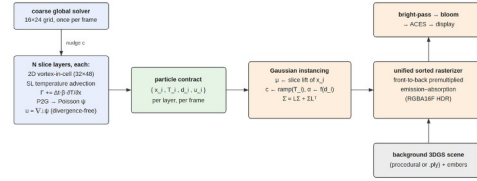
Figure 2. System overview. A coarse global vortex solver drives N per-slice 2D vortex-in-cell simulations (left, §4). Each slice exposes its particles through a minimal contract (center); the renderer lifts each particle directly into an emissive anisotropic Gaussian (§5) and rasterizes all Gaussians—fire, smoke, embers, and the background 3DGS scene—in one depth-sorted emission–absorption pass with HDR post-processing. There is no voxelization or resampling anywhere in the pipeline.
