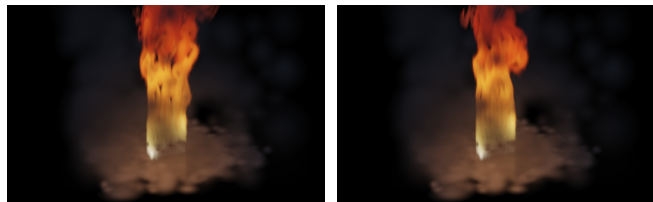
Fig. 15. The inter-slice exchange operator, seen rather than plotted: same seed, same step count, world-fixed slices from a 63^\circ side view (turbulence, wind and coarse coupling disabled to isolate the operator). Left ( \kappa_z=0 ): each slice burns as an independent flame with its own hot core—the stack reads as separate sheets. Right ( \kappa_z=0.45 ): the pairwise circulation exchange fuses the bases into one core and the bodies into one connected volume, the visual counterpart of \rho : 0.18 \rightarrow 0.62 (§7).
