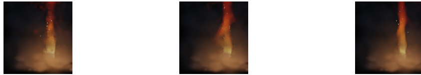
Figure 7. Covariance dynamics. Left: isotropic splats ( k_z=0 ) read as soft blobs. Middle: flow-driven covariance (Eq. 5) shears splats into flame licks. Right: adding the trajectory filament stretch (Eq. 6) elongates fast particles into path-aligned streaks.
