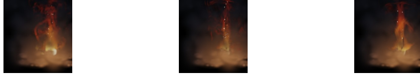
Figure 8. Covariance dynamics. Left: isotropic splats ( k_z=0 ) read as soft blobs. Middle: flow-driven covariance (Eq. 5) shears splats into flame licks. Right: adding the trajectory filament stretch (Eq. 6) elongates fast particles into path-aligned streaks.
