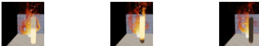
Figure 3. Fire spread on the scene’s own primitives (§5.6), one continuous simulation. Left ( t \approx 2.5 s): a single ignition at the front pillar’s base; the fire line climbs the pillar while the loop already feeds a plume that curls around it. Middle ( t \approx 7.5 s): the pillar is engulfed—burning splats glow in HDR, shed embers, and spawn flame particles into the slice solvers. Right ( t \approx 16.5 s): the front pillar is consumed—char written into the splats’ albedo and opacity—and the plumes it emitted have carried heat across a \sim 1.7 -unit gap and ignited the rear pillar, far beyond the splat-graph’s spread radius: the jump happens through the simulated flame, not the adjacency graph. The ground is marked non-flammable (zero fuel).
