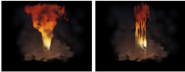
Fig. 8. Slice orientation. Same simulation state, seed, camera and shading; only the slice frame differs. The camera sits at a 79^\circ orbit—close enough to the slice planes’ edge to expose the degeneracy, oblique enough that the individual planes are still distinguishable. Left : view-aligned slices re-orient with the camera, so the stack integrates into a volume and reads correctly from any azimuth. Right : world-fixed slices seen near edge-on separate into the flat sheets they actually are—the plume loses its silhouette and becomes nine ribbons standing on the ground. At exactly 90^\circ they collapse further, into single-pixel lines. This is the failure mode that motivates view alignment, and the reason a Lagrangian state that can be re-sliced per frame at no re-simulation cost is worth having.
