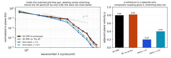
Fig. 13. Ablating the layered decomposition’s missing term inside an otherwise identical solver (§7). The 3D Gaussian vortex-particle solver runs in the shipping prototype and shares the kernel family, core radius, opening angle, particle scheme, source terms, timestep, mapping and renderer with the slice stack, and is sampled on the same nine planes through the same protocol. Left : under the grid-free pair the stack’s spectral gap to matched 3D is modest (log- L_1 0.28–0.40), and switching off vortex stretching (\alpha \cdot \nabla)\mathbf{u} inside the 3D solver moves its spectrum by only 0.06—under this discretization, most of the residual gap is the loss of three-component transport coupling, not the stretching cascade. (The retained grid-based pair had attributed \sim 70\% of a far larger gap to stretching: the attribution is discretization-dependent, which is itself a finding.) Right : z -coherence remains the stack’s clearest deficit: adjacent-plane \rho = 0.80 for 3D against 0.20 (uncoupled) / 0.40 (coarse-coupled) for the stack; the inter-slice exchange of Eq. 8 recovers most of it (§7). Any future inter-slice operator must be measured on both axes.
