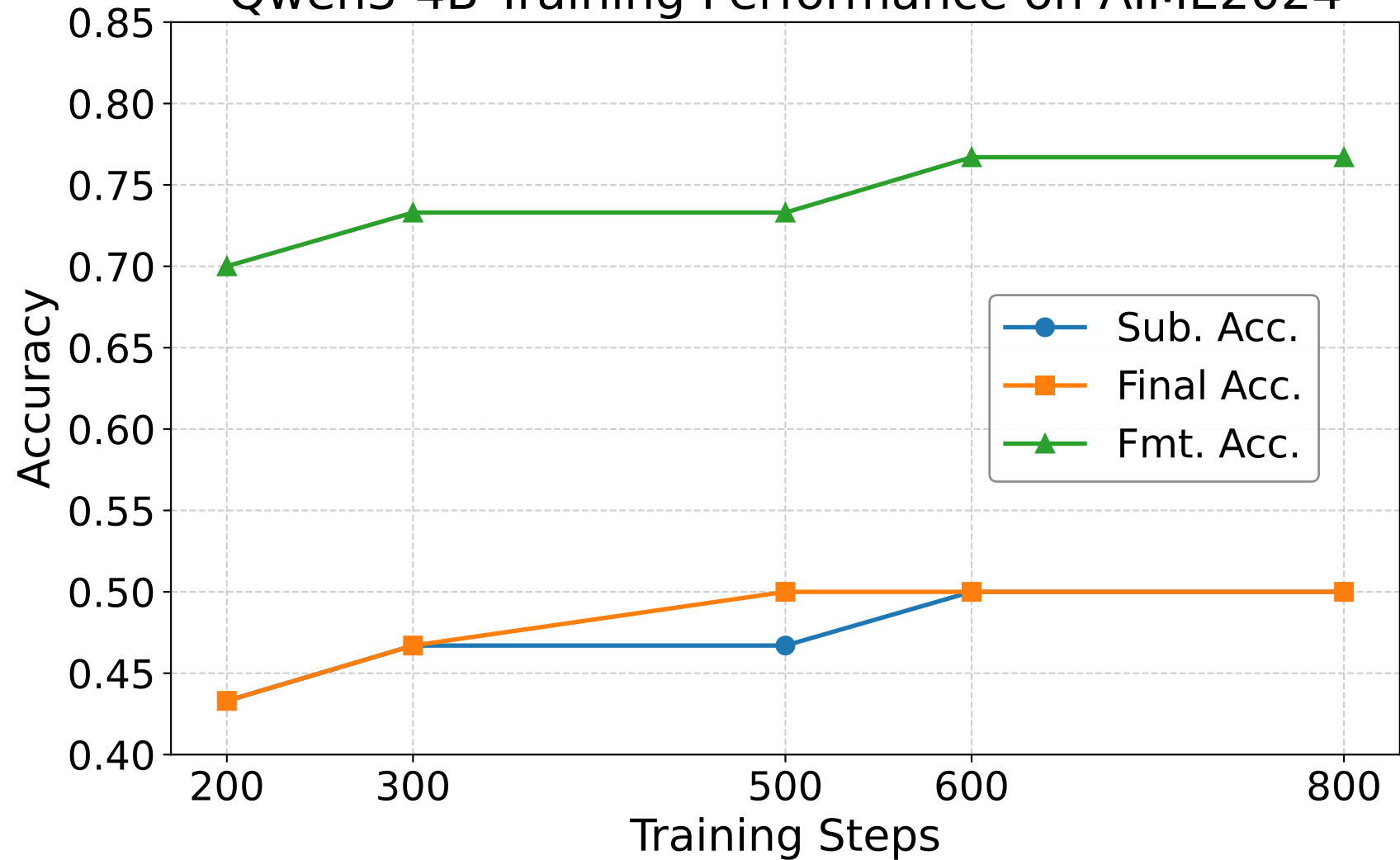
Qwen3-4B Training Performance on AIME2024
