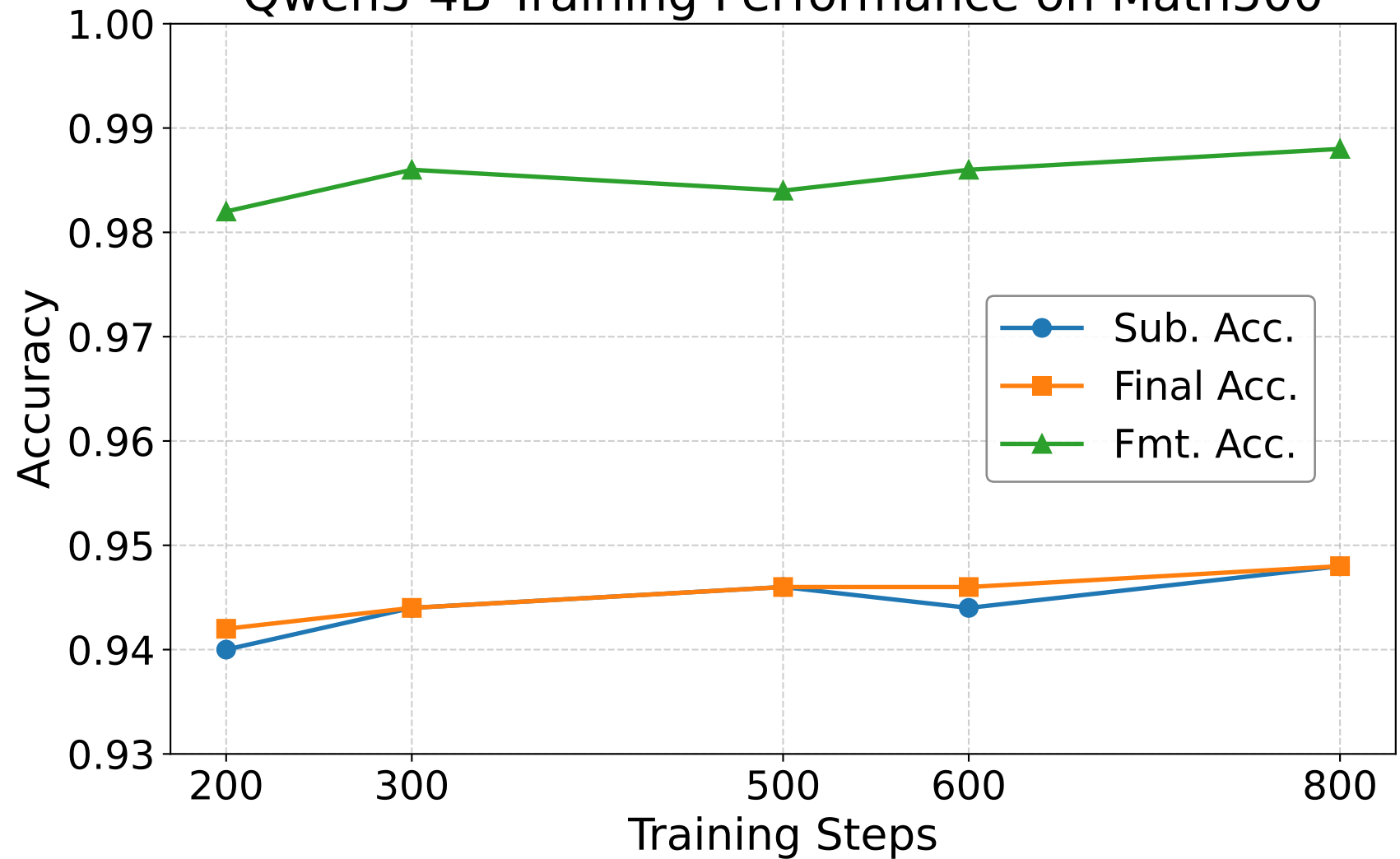
Qwen3-4B Training Performance on Math500
