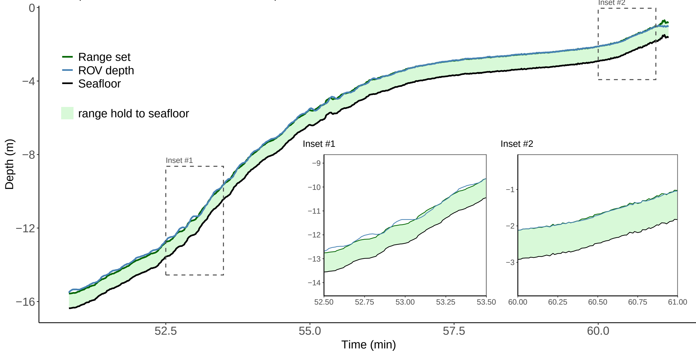
ROV depth relative to seafloor and surftrak setpoint
