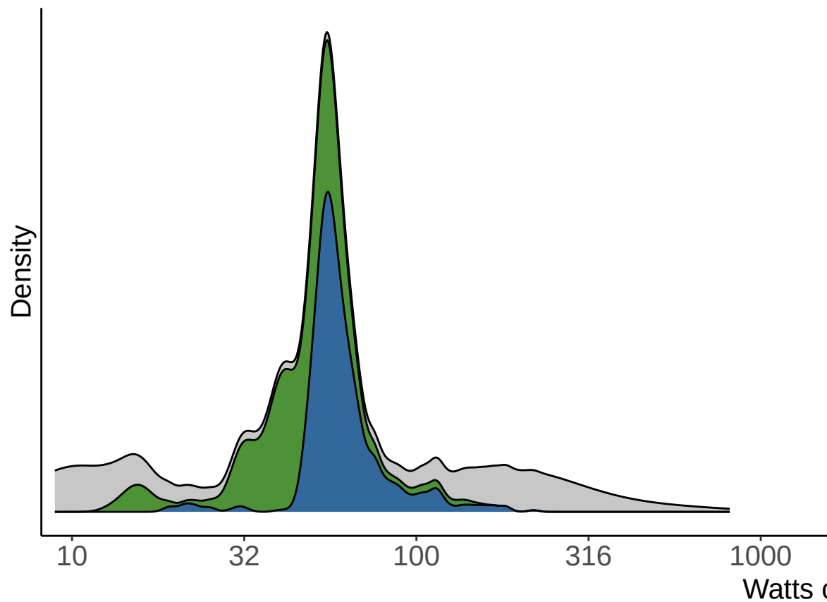
0–1 kt water current
