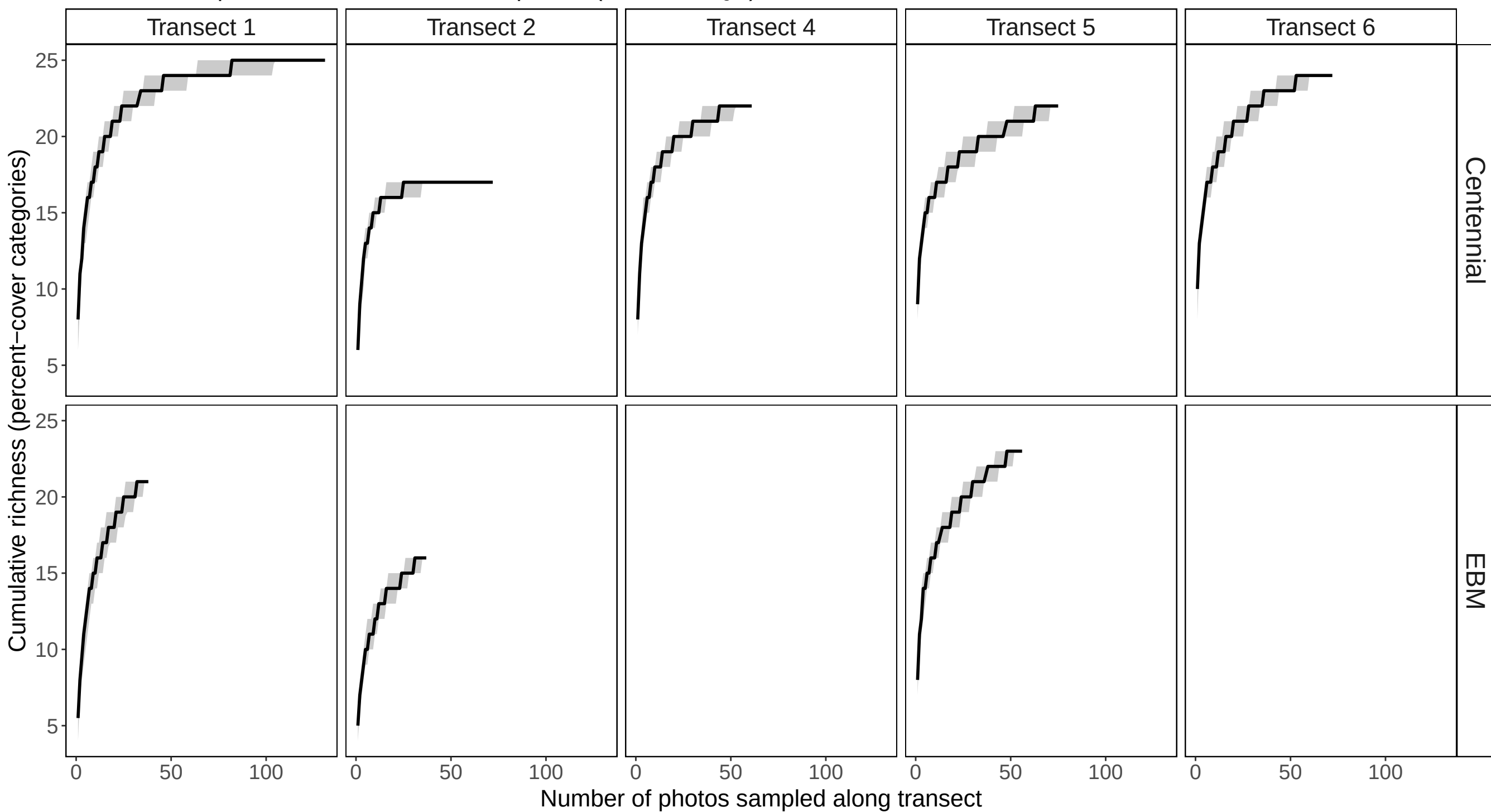
Randomized species accumulation across photos (median \pm IQR)
