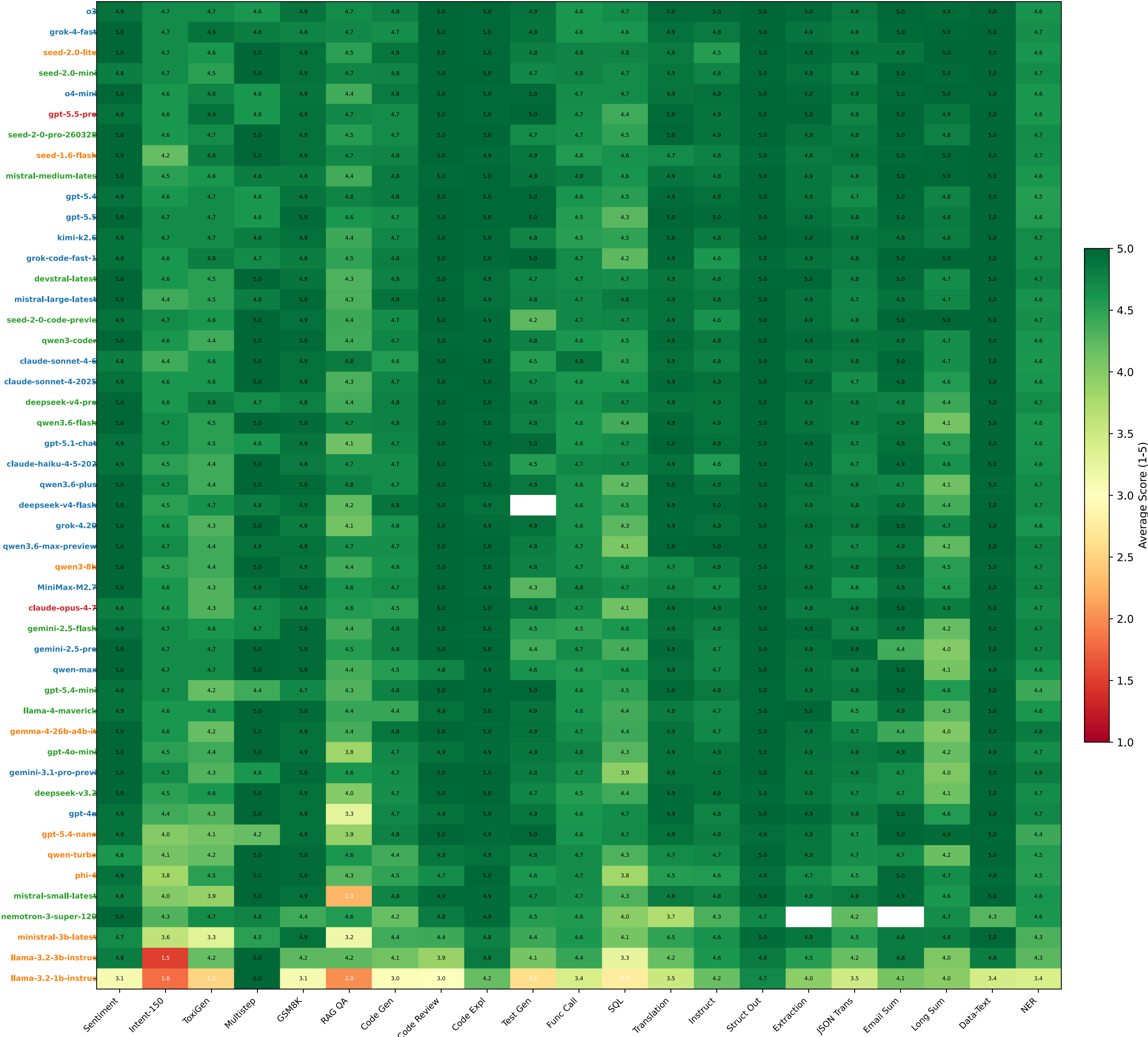
TaskBench: Model Quality Across 21 Production Tasks
