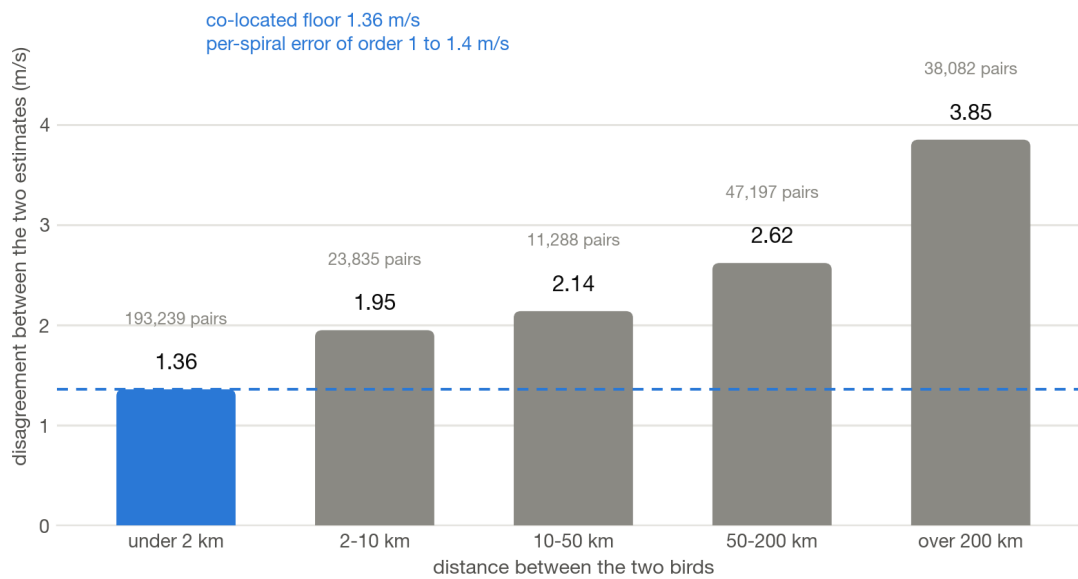
Figure 3: Disagreement between two independent wind estimates against the distance separating the two birds, 19,565 spirals from 60 white storks. Noise would give the same value at every distance.
