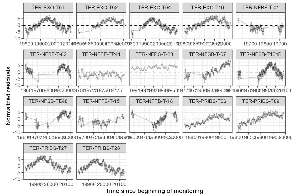
UND_temperature_mean — residuals through time
