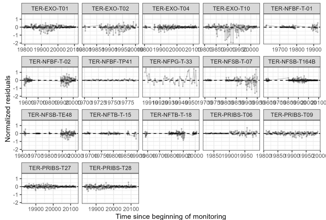
CAN_DVPDR — residuals through time
