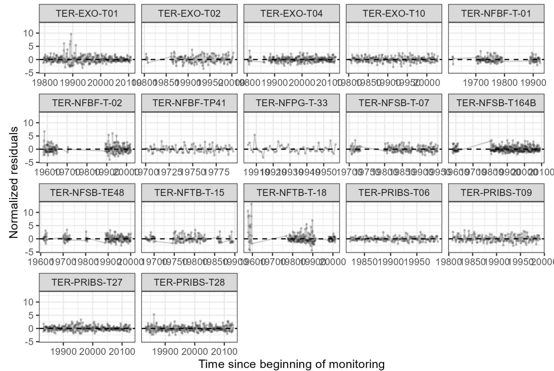
GRD_DTR — residuals through time
