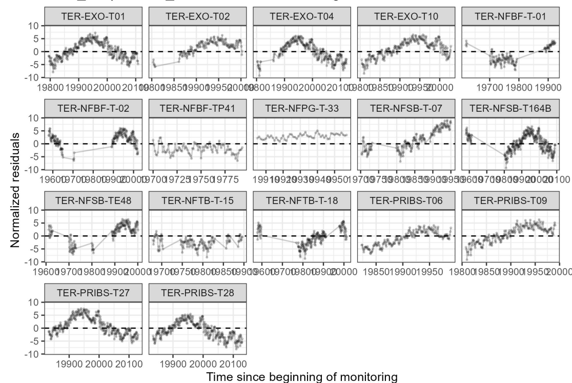
GRD_temperature_mean — residuals through time
