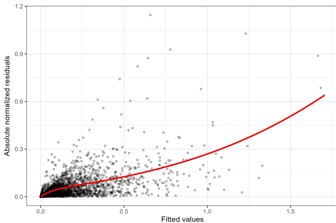
GRD_DVPDR — scale-location plot
