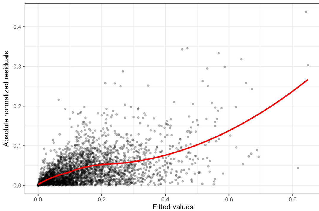
UND_vpd_kPA_mean — scale-location plot
