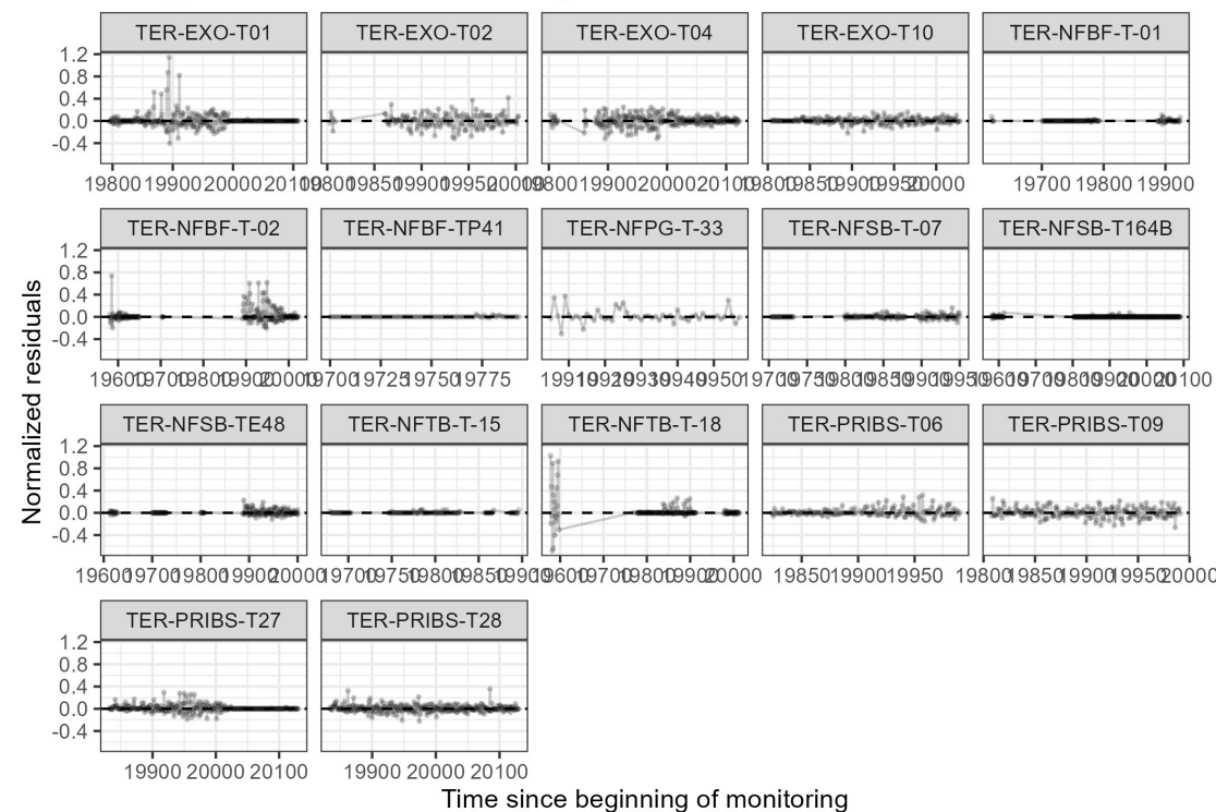
GRD_DVPDR — residuals through time
