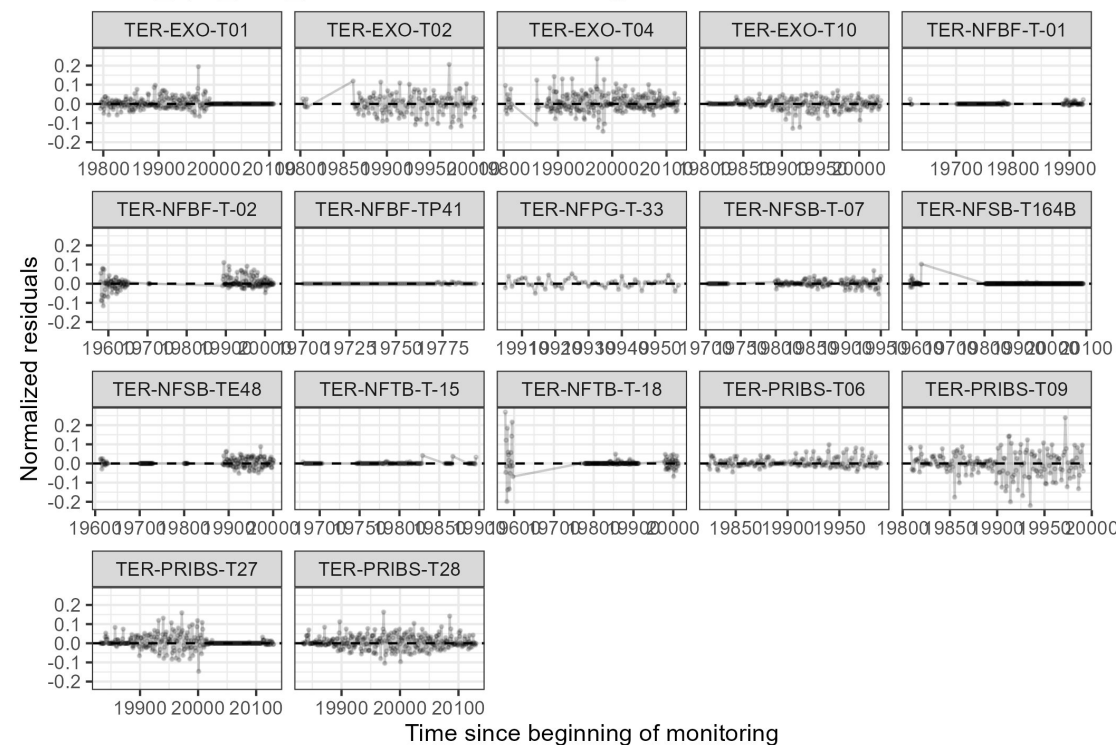
GRD_vpd_kPA_mean — residuals through time
