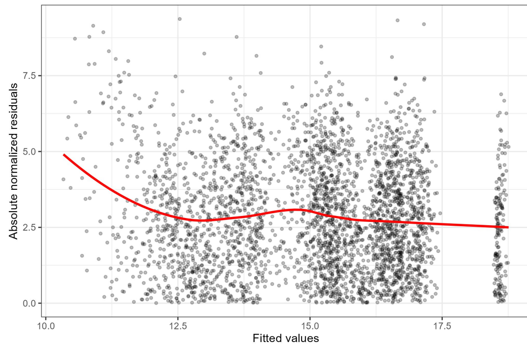
GRD_temperature_mean — scale-location plot
