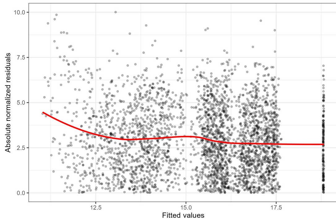
CAN_temperature_mean — scale-location plot
