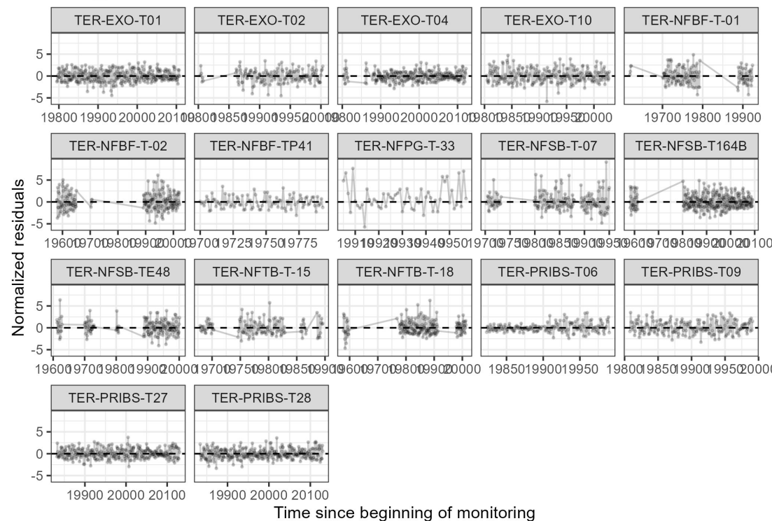
CAN_DTR — residuals through time
