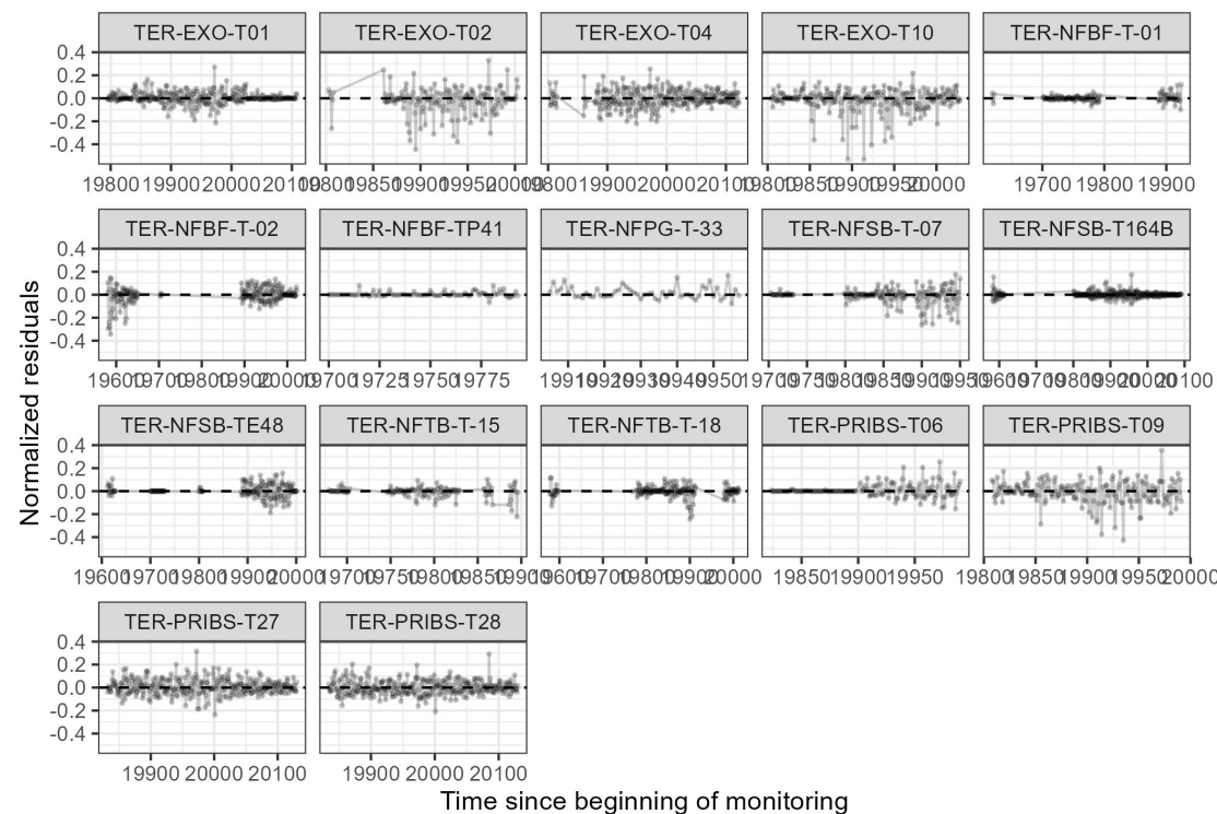
CAN_vpd_kPA_mean — residuals through time
