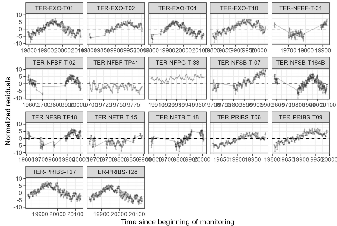
CAN_temperature_mean — residuals through time
