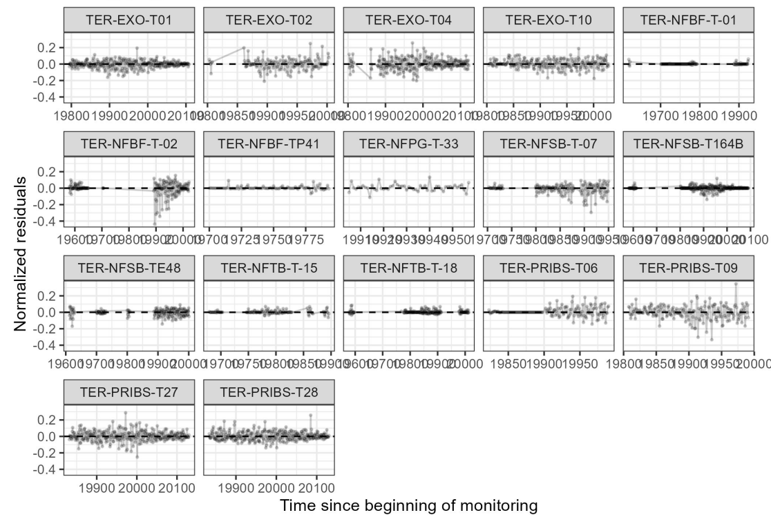
UND_vpd_kPA_mean — residuals through time
