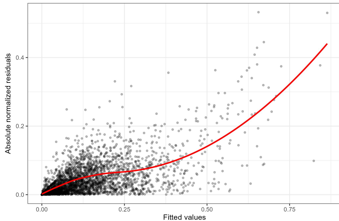
CAN_vpd_kPA_mean — scale-location plot
