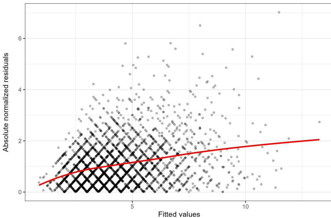
UND_DTR — scale-location plot
