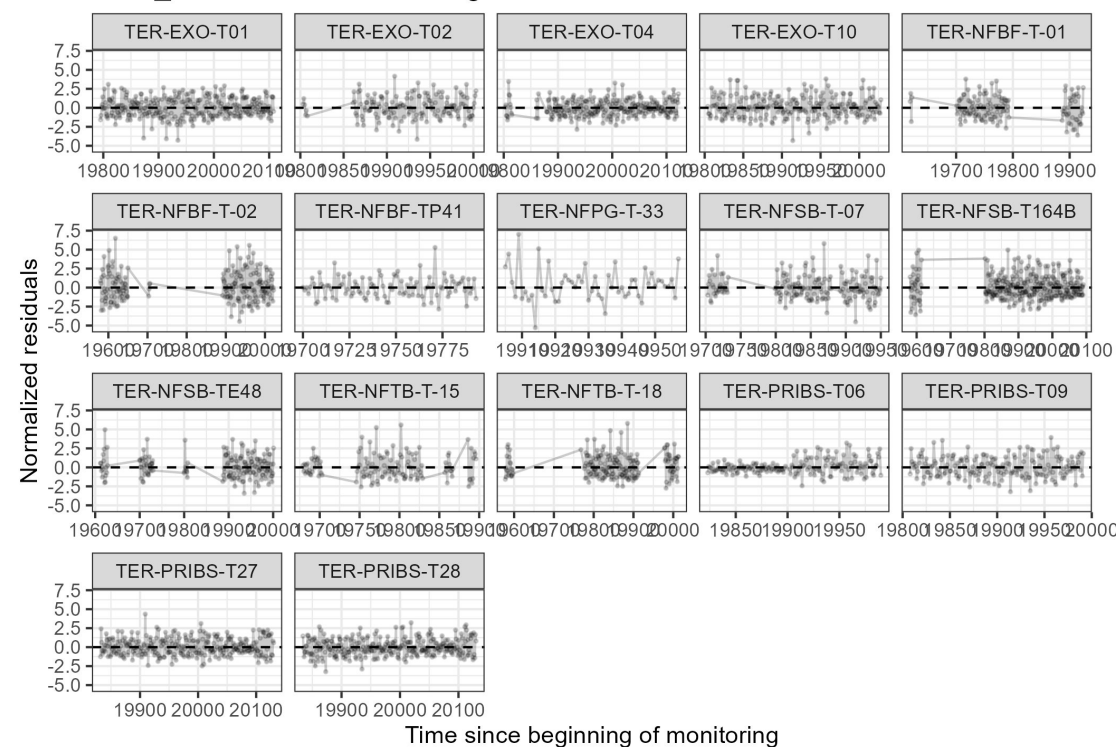
UND_DTR — residuals through time
