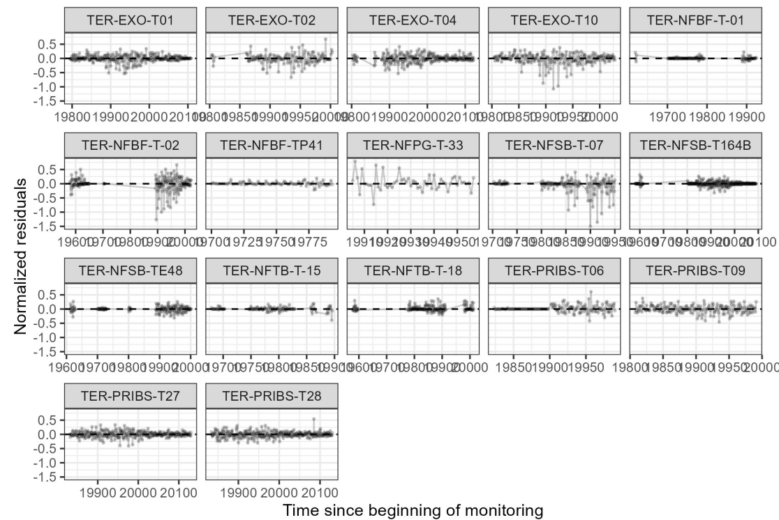
UND_DVPDR — residuals through time
