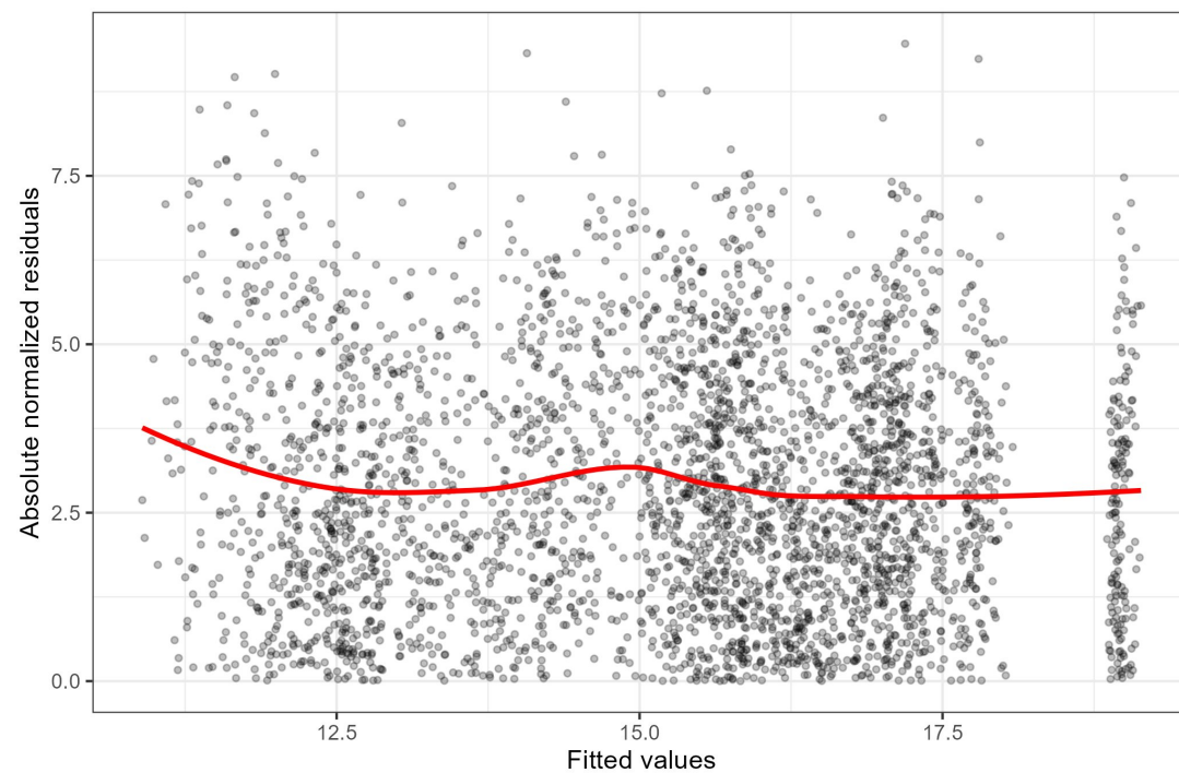
UND_temperature_mean — scale-location plot
