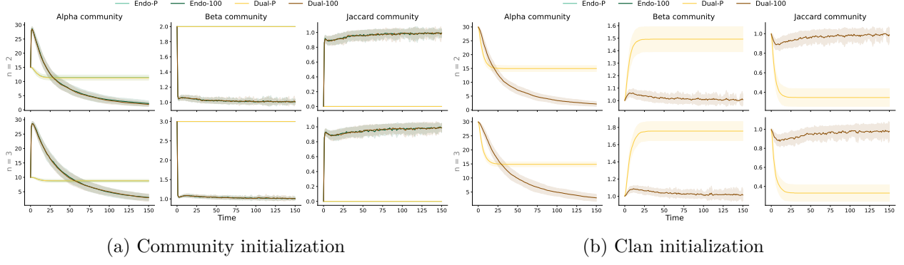
Figure 3: Community richness measures for all configurations
