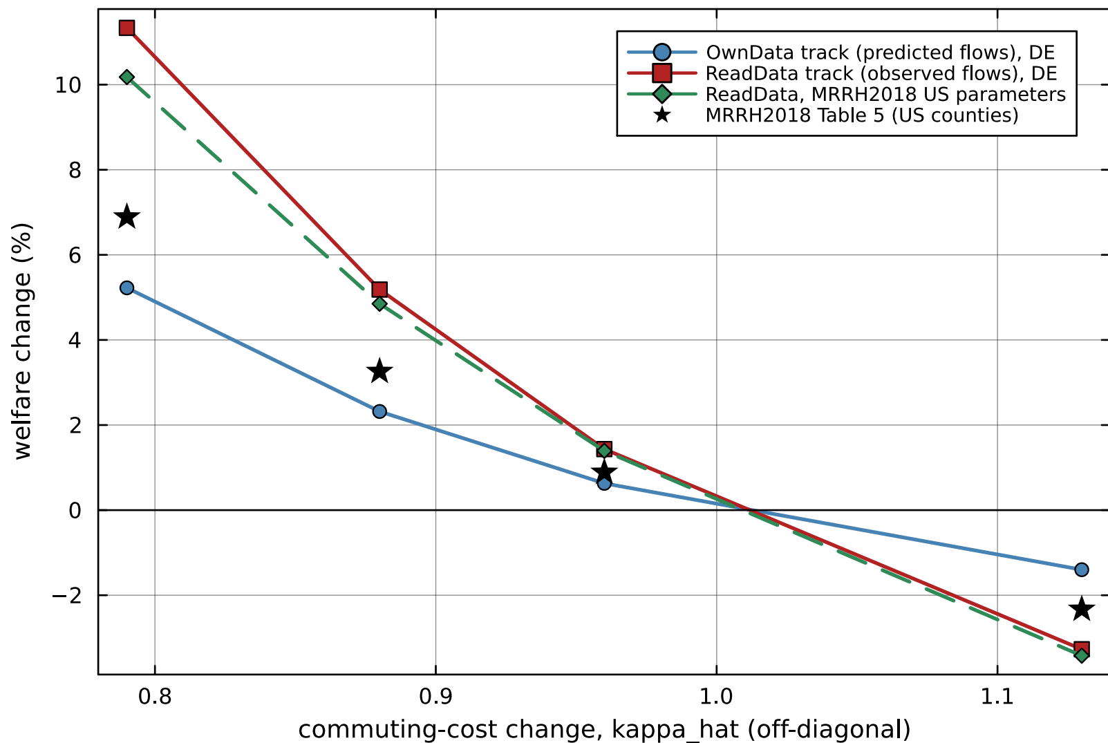
MRRH2018 Table 5 experiment, reproduced on German counties
