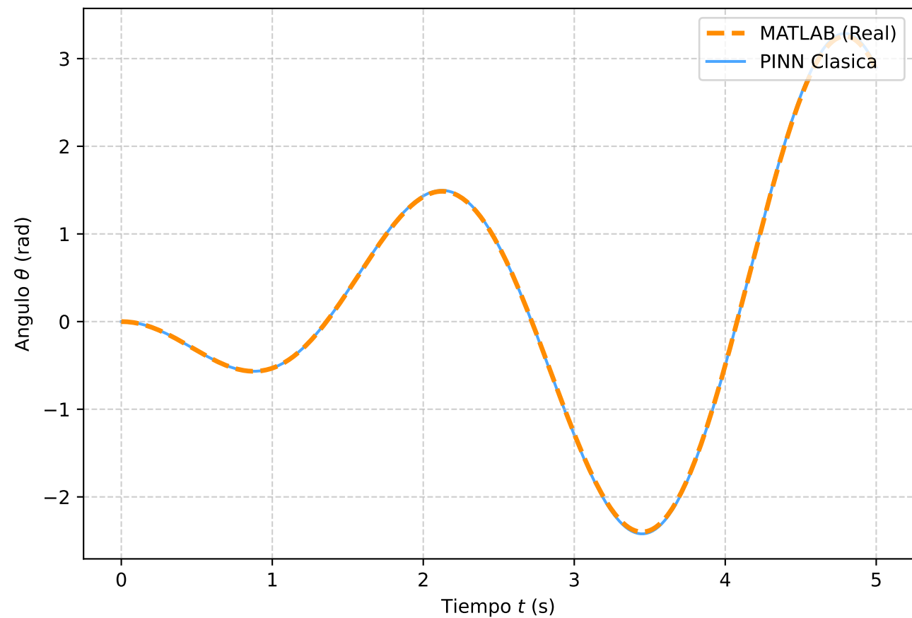
Movimiento Torsional \theta(t) - [0 a 5s]
