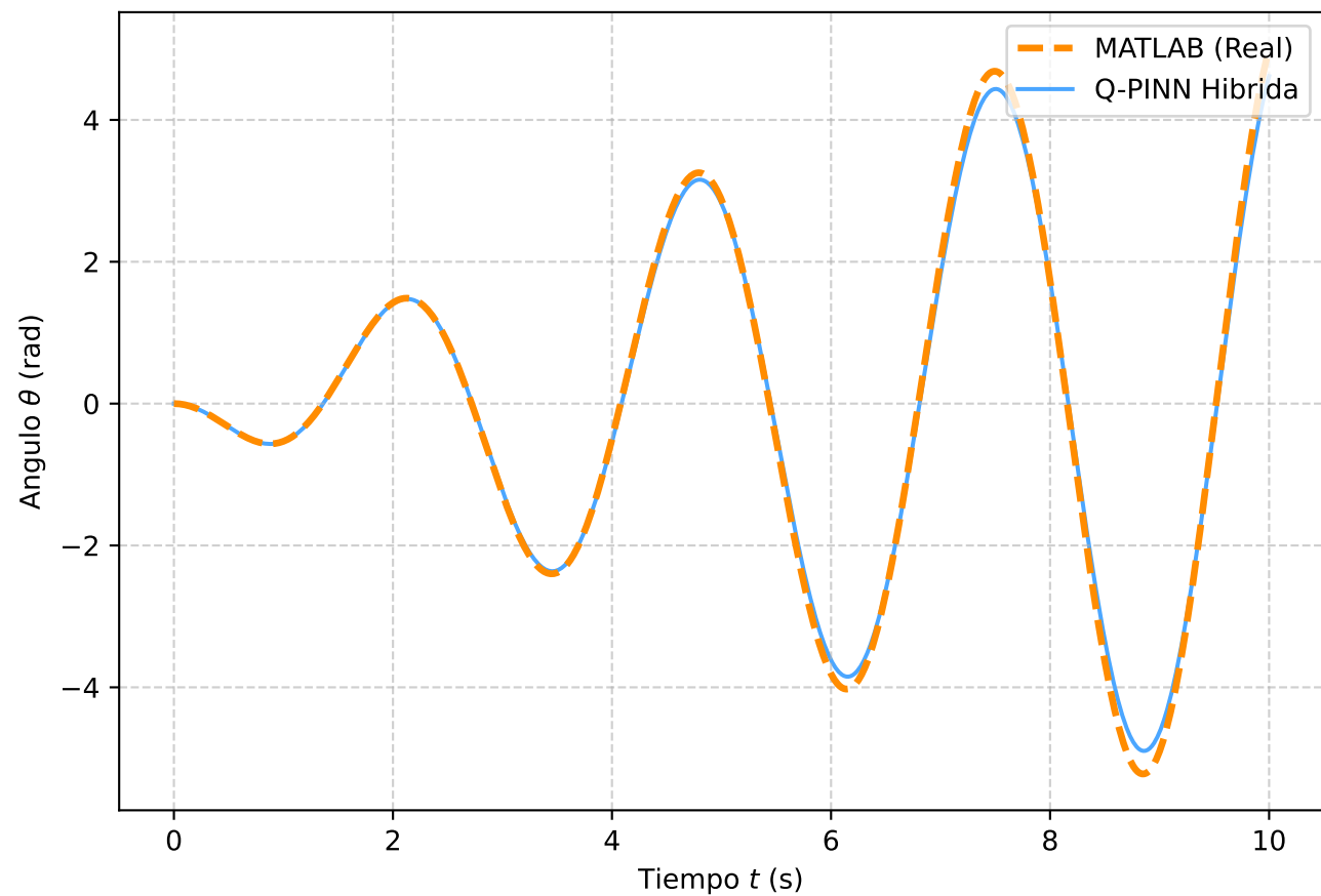
Movimiento Torsional \theta(t) - [0 a 10s]
