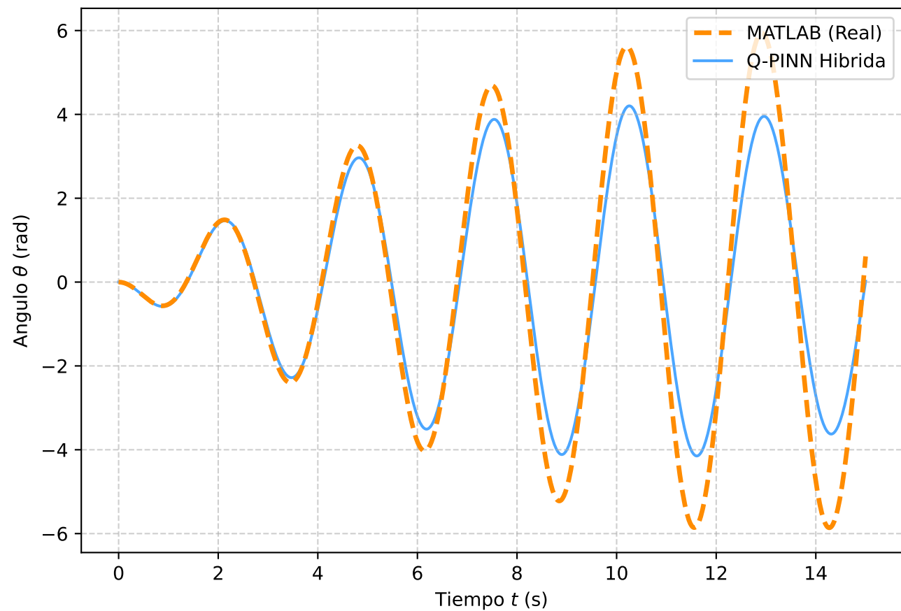
Movimiento Torsional \theta(t) - [0 a 15s]
