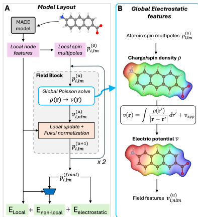
Fig. 2. MACE-POLAR-1 (Batatia et al. , 2026).
