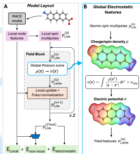
Fig. 2. MACE-POLAR-1 (Batatia et al. , 2026).
