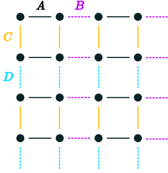
FIG. 17. Grouping of interactions, which commute within the group.
