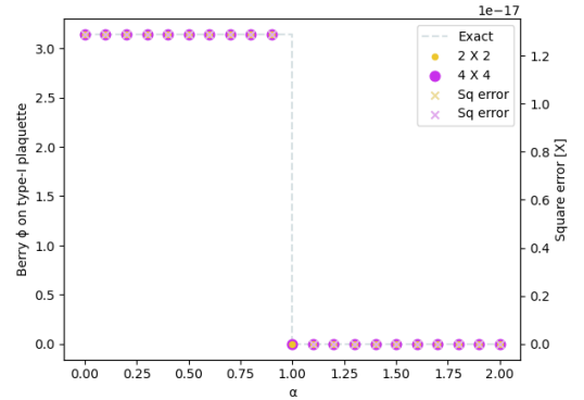
FIG. 18. Berry phase for 2x2 and 4x4 systems, computed in-silico, via Hamiltonian decomposition, and loop unitary evolution.
