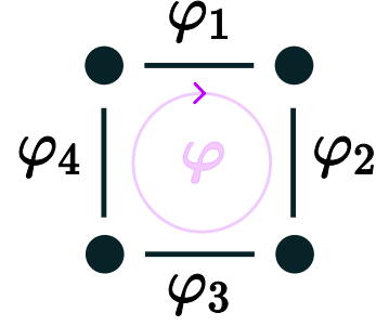
FIG. 15. Plaquette twist on each link.
