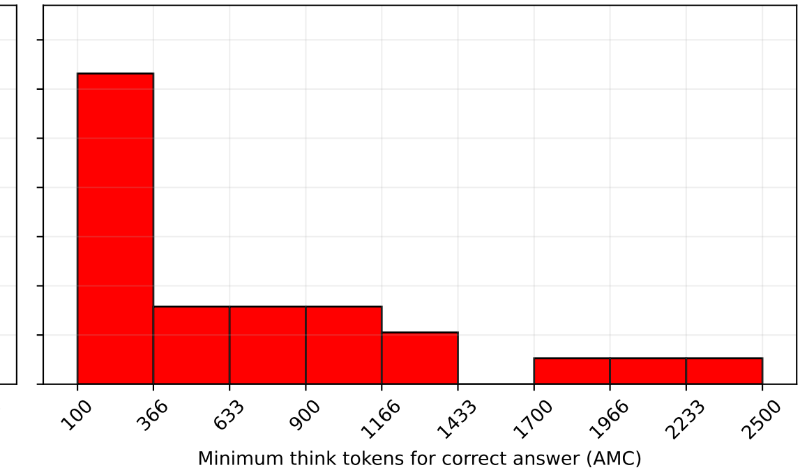
AMC
