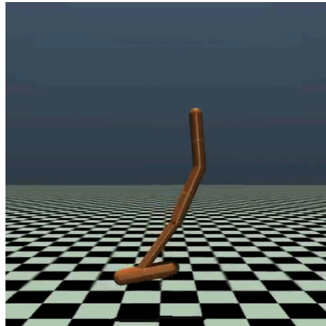
Hopper (SAC).
