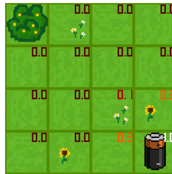
In-place iterative policy evaluation
