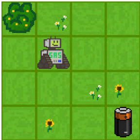
Gridworld
