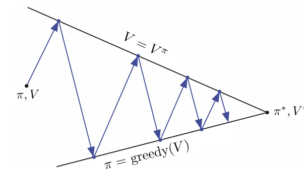
GPI (Sutton and Barto 1998)
