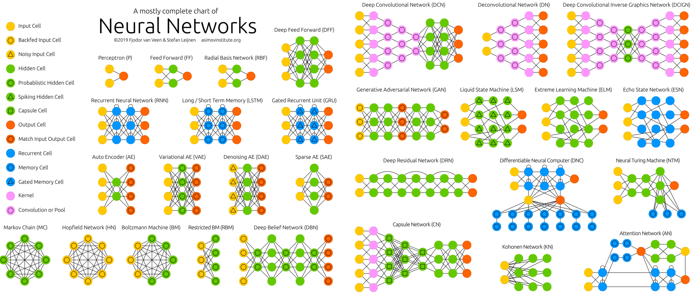
The neural network zoo [Asimov Institute].
