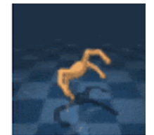
Quadruped Run
