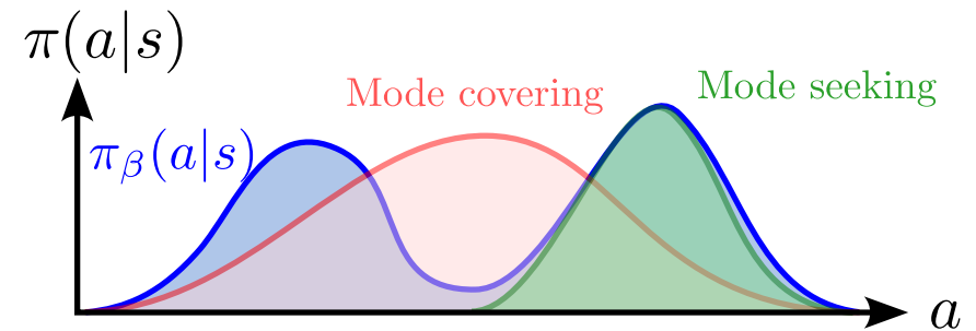
Mode seeking vs. mode covering (inspired by Sergey Levine's CS285 lecture ).
