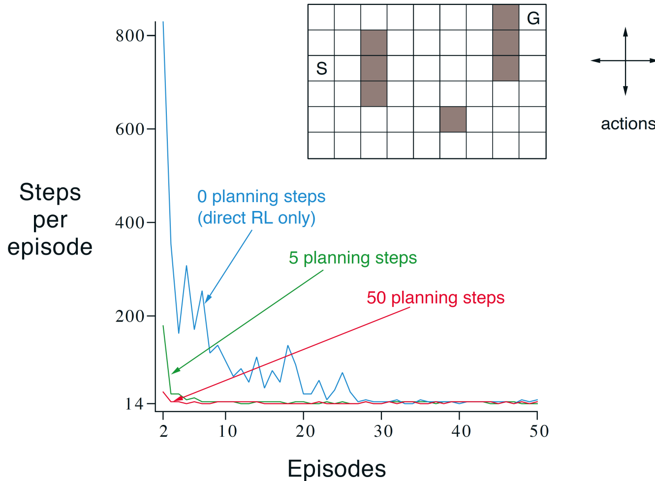
A simple maze (inset) and the average learning curves for Dyna-Q agents varying in their number of planning steps ( n ) per real step. The task is to travel from S to G as quickly as possible (Source: (Sutton and Barto 1998, Fig. 8.2)).
