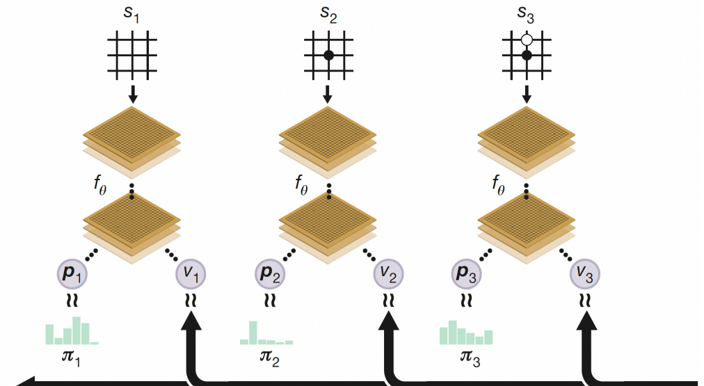
(1) Neural network training
