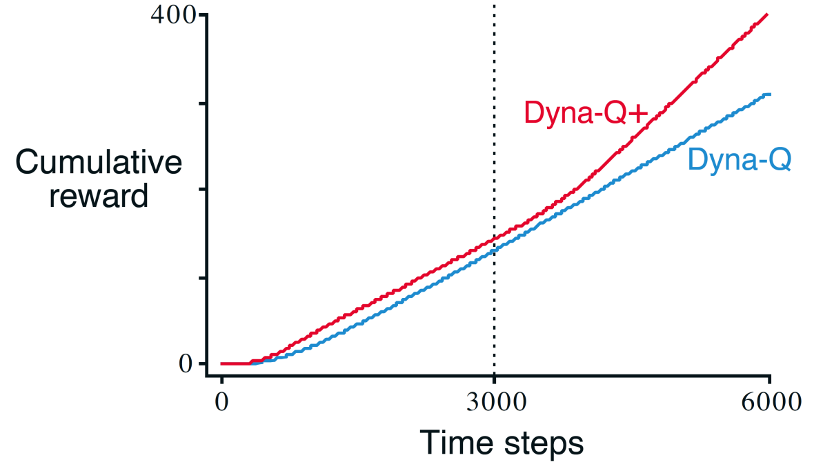
Average performance of Dyna agents on a shortcut task. The left environment was used for the first 3000 steps, the right environment for the rest (Source: (Sutton and Barto 1998, Fig. 8.5)).
